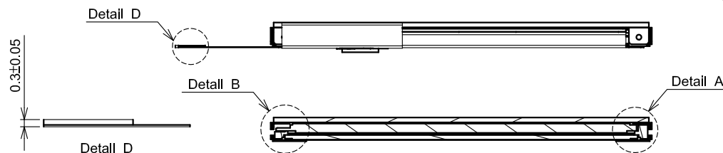
SECTION H2-H2
