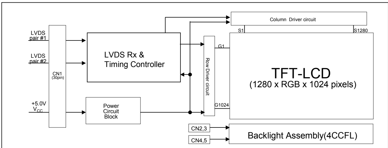
Figure 1. Block diagram
